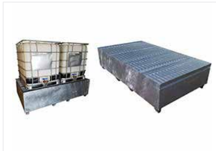
IBC TWIN BANDED PALLET - GALVANISED 550mm H x 1320mm L x 2250mm D
