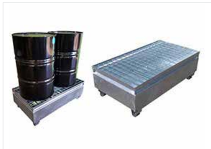
2 DRUM - GALVANISED 400mm H x 1220mm L x 670mm D
