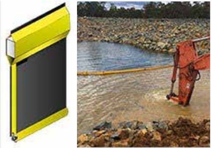
SILT CURTAIN - CLASS 1 CONTACT US FOR A QUOTE Low-Risk Applications Little to no tidal, wave and/or wind forces. Example: lagoon, pond, stream.
